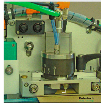
CorruTack - Board Gluing System
