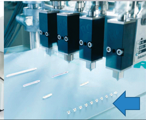
CorruTack - Board Gluing System
